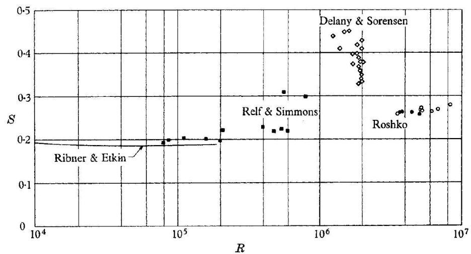
Figure 19: Strouhal number of vortex shedding frequency
